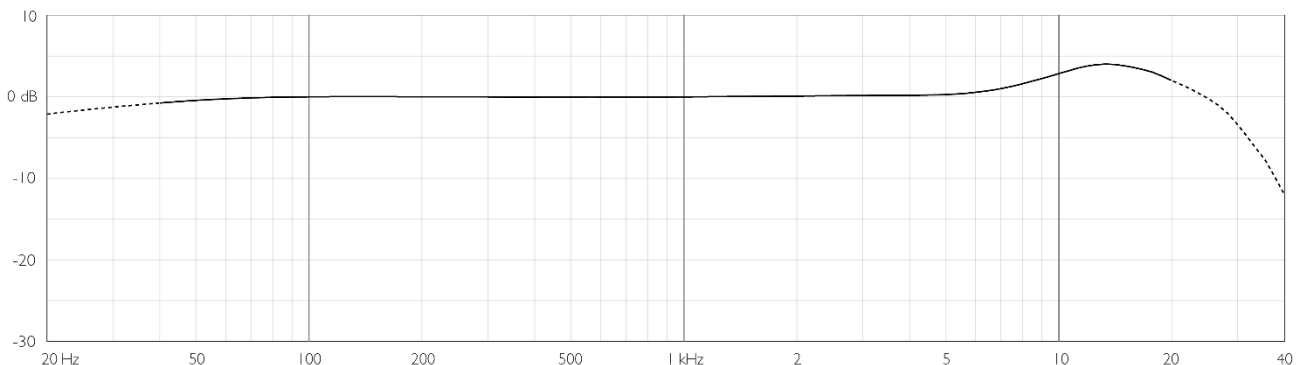
6066 Frequency response
