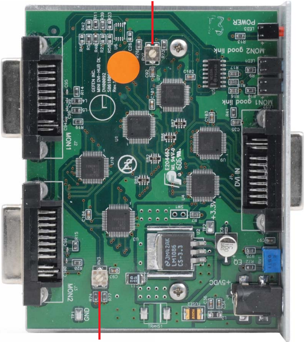
Internal Equalization Knob for DVI Output 2
